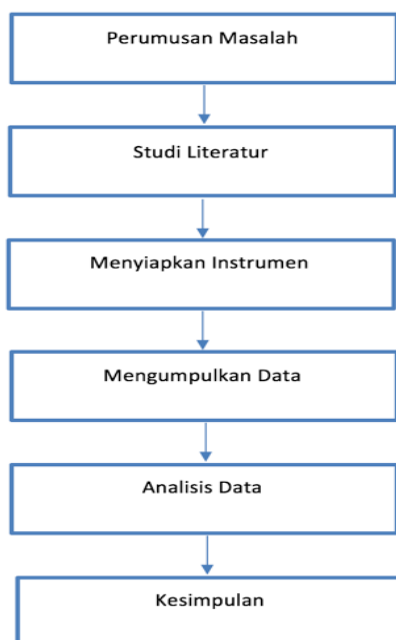
Gambar 1 Metode Penelitian
